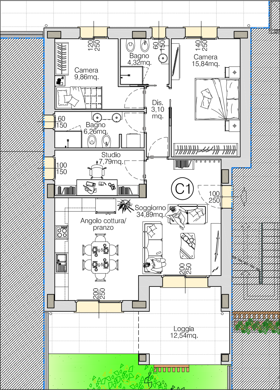
PIANO TERRA
