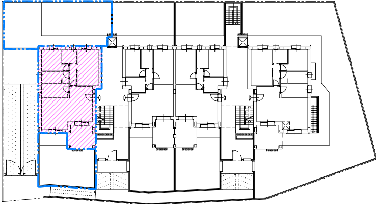
PIANO TERRA
